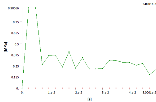
Gambar 18. Grafik equivalent stress
