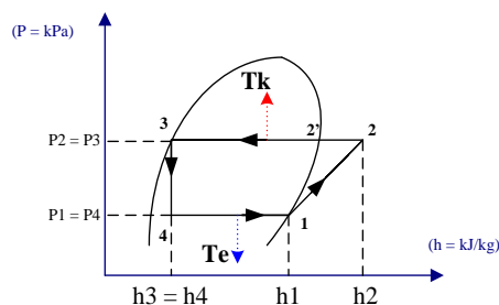
Gambar 4.1 P-h Diagram
