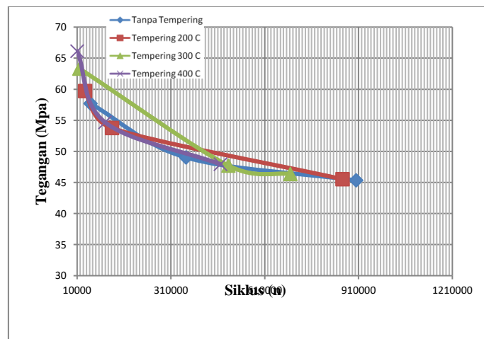
Gambar 4 Diagram S-N Paduan Aluminium-Magnesium
