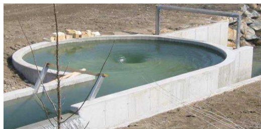
Gambar 2.5 Turbin vortex Zotloterer
