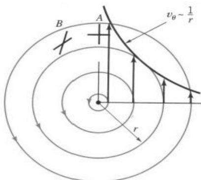
Gambar 2.2 aliran irrotational
