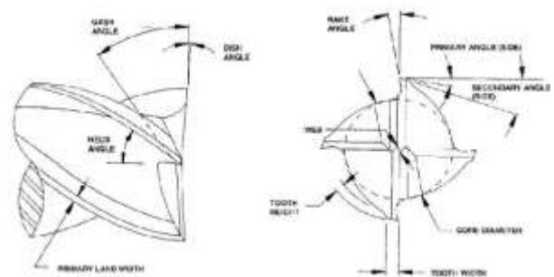
Gambar 3. Geometri Sisi Potong Endmill cutter
