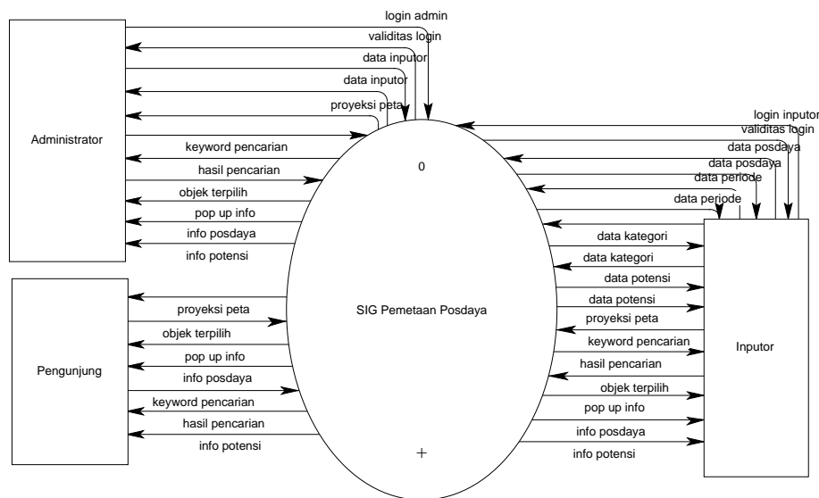
Gambar 4. DFD Level 0 SIPODA
