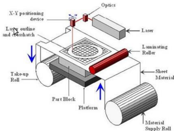
Fig. 2 Laminated Object manufacturing schematic
