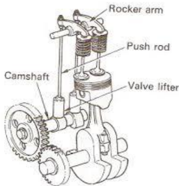
Gambar 3: Timing Gear
