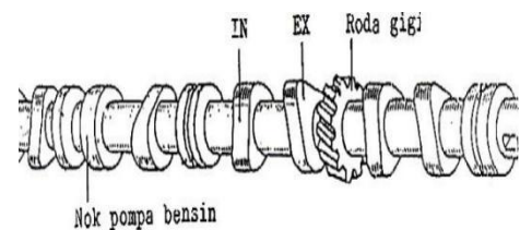
Gambar 11: Poros Nok
