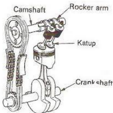
Gambar 4: Timing Chain
