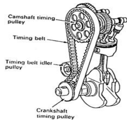
Gambar 5: Timing Belt
