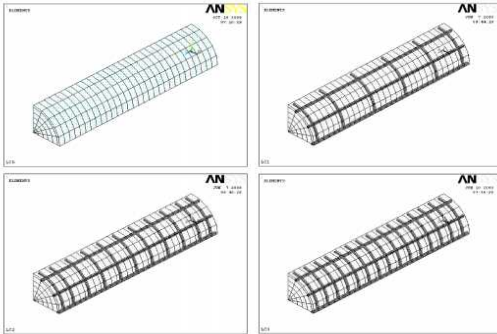
Figure 6. Element meshing of quarter column specimens LC0, LC1, LC2, and LC3
