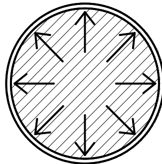
Figure 1. Effective confined regions in a concrete core of a circular column cross section
