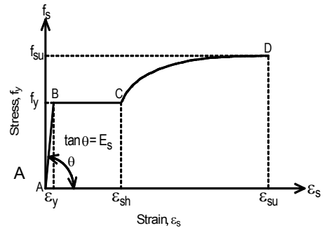
Figure 5. Stress-strain relationship for reinforcing steel proposed by Park and Paulay [22]
