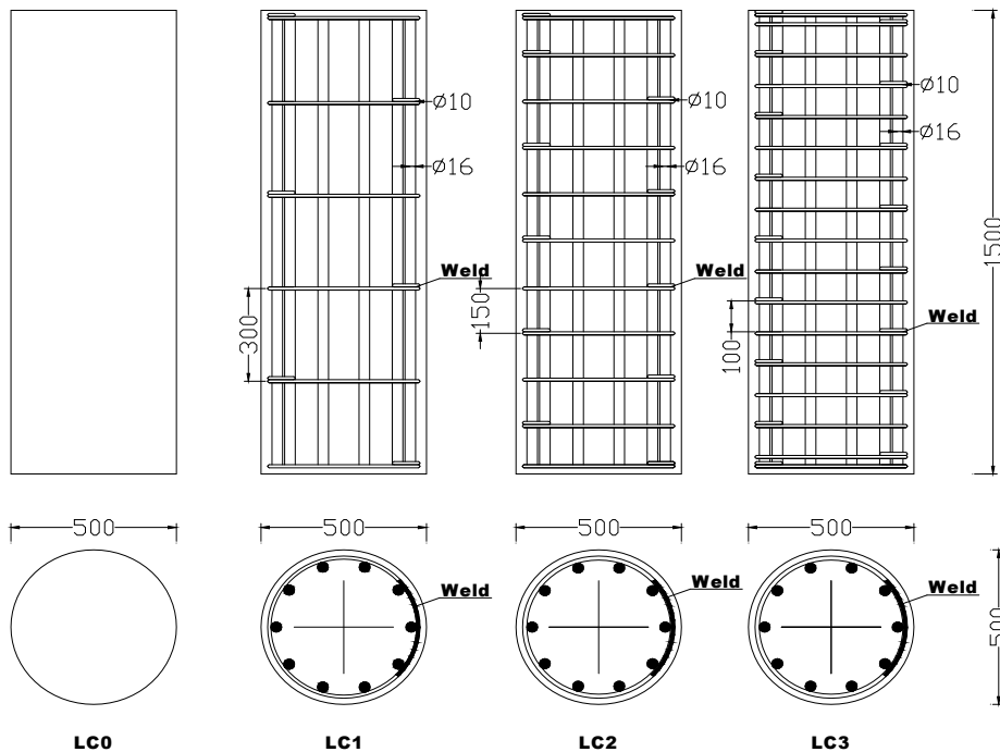
Figure 3. Geometrical properties of column specimens LS0, LS1, LS2, and LS3 used for model validation
