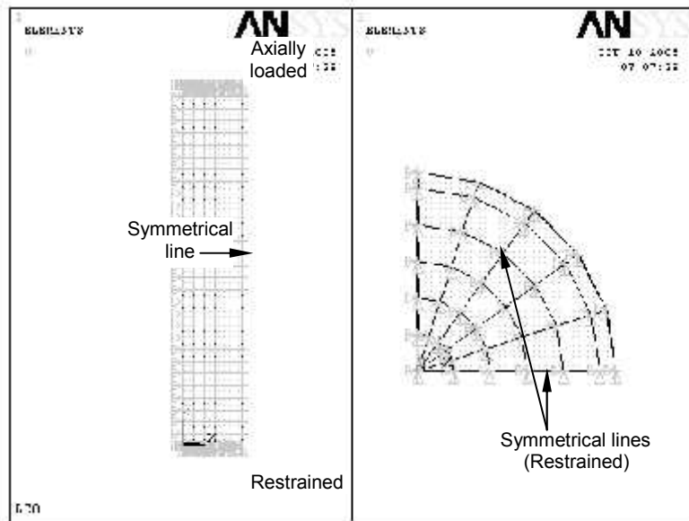
Figure 2. Boundary conditions of a symmetrical quarter of a column model: (a) elevation; (b) cross section
