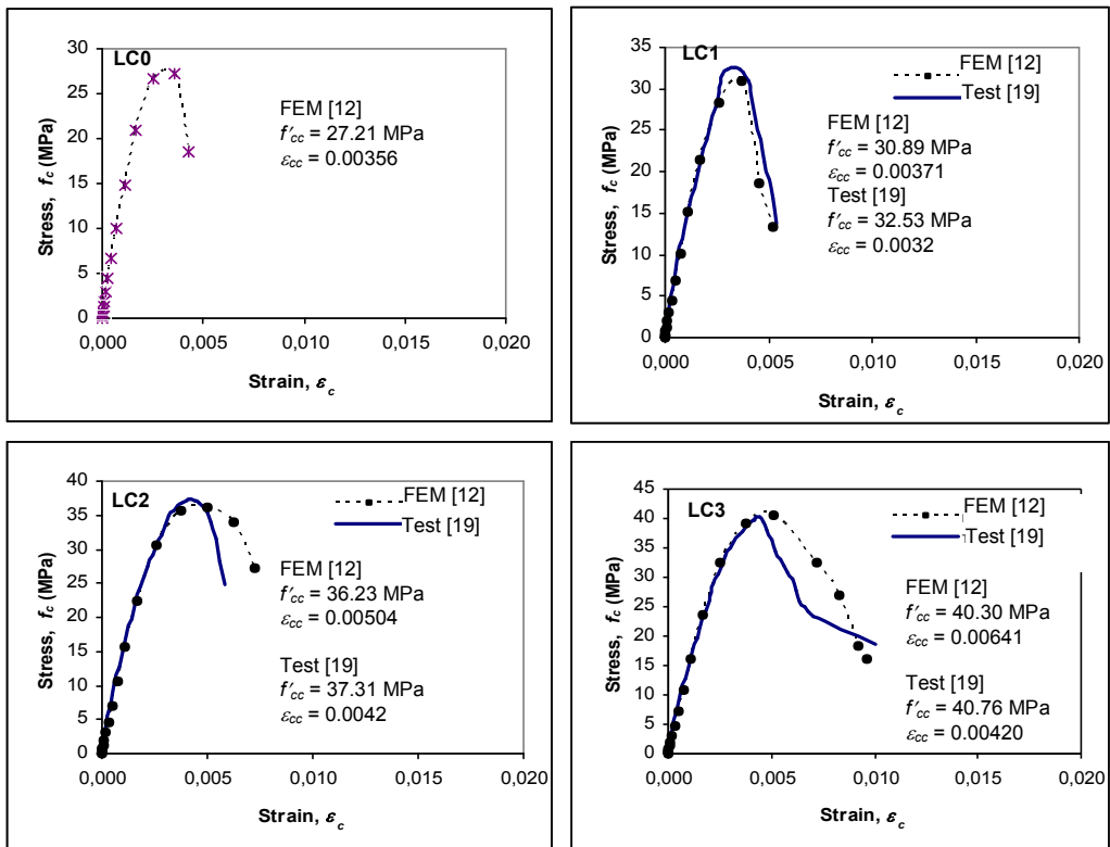
Fig. 8. Stress-strain curves of column specimens LC0, LC1, LC2, and LC3
