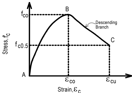
Figure 4. Stress-strain relationship of concrete proposed by Popovics [20,21]
