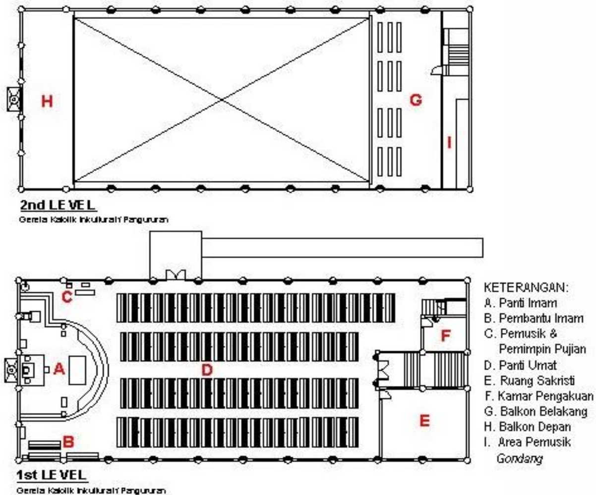
Gambar 5. Layout interior GKIP
