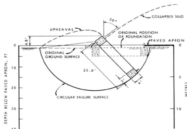
Figure 3. Attitude of a silo foundation after failure.
