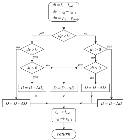
Figure 3. Improved P & O algorithm flowchart as shown in [2]
