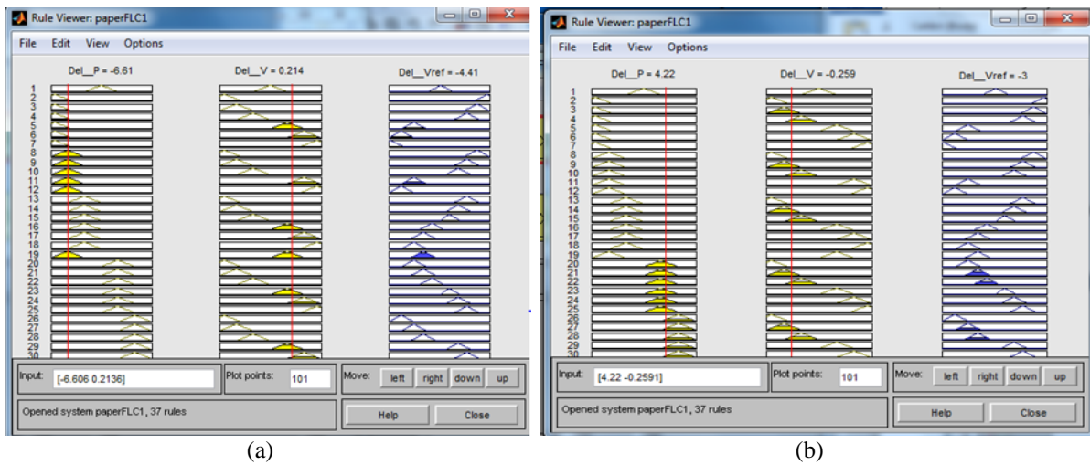
Figure 7. Rule viewer of the designed new fuzzy logic controller: (a) IP1 (Del_P) is negative side, (b) IP2 (Del_V) is negative side
