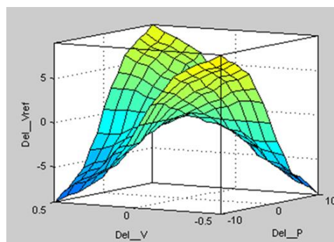
Figure 8. Surface view of designed new fuzzy logic controller
