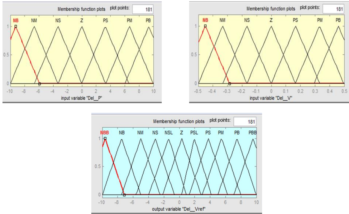
Figure 6. Membership function of the fuzzy logic control MPPT approach (a) Del_P (b) Del_V (c) Del_V ref
