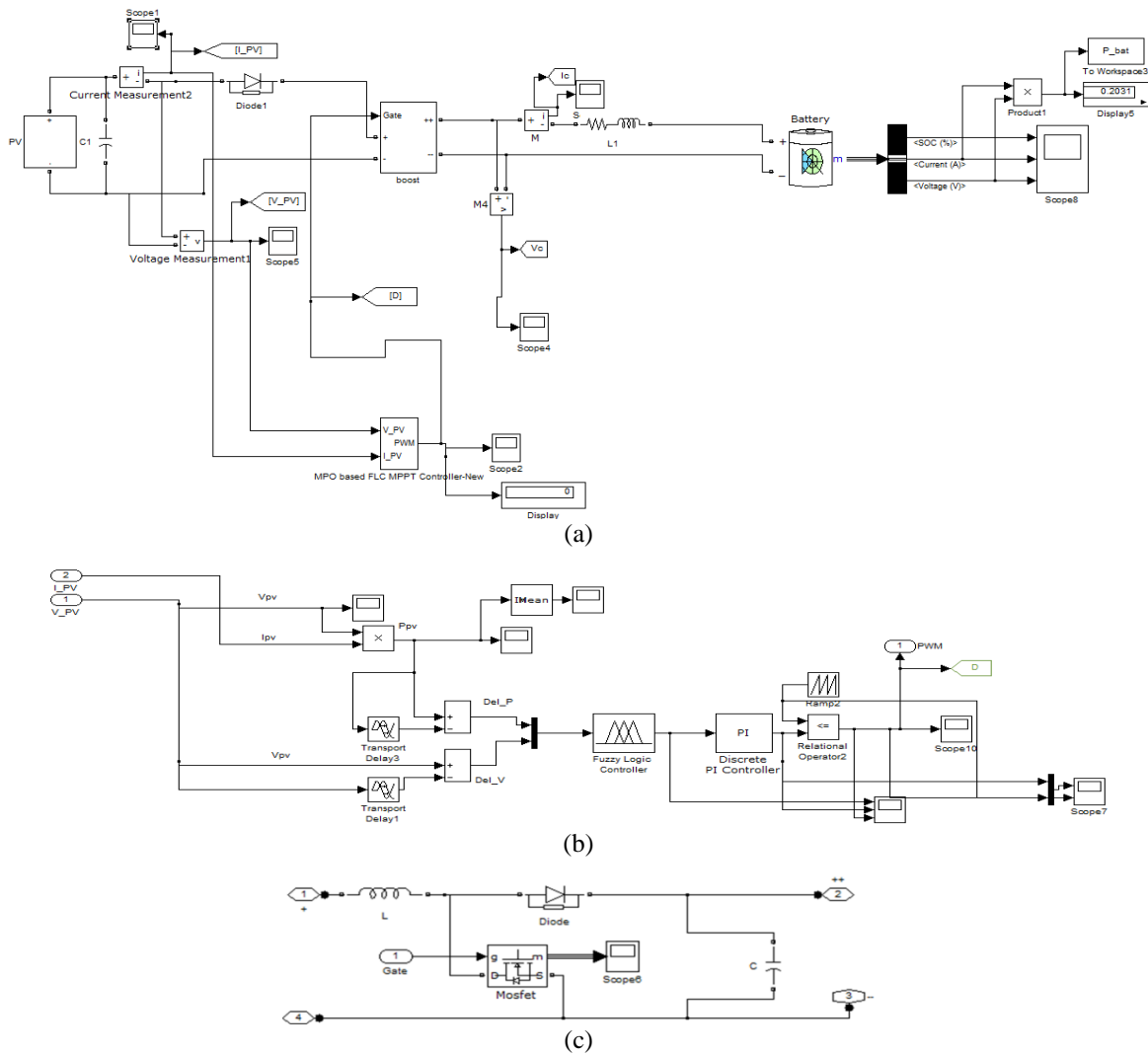
Figure 4. (a) proposed overall setup of the PV system (b) Subsystem of the Fuzzy logic controller (c) DC to DC Boost converter
