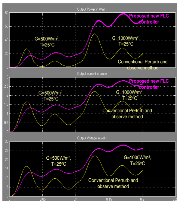
Figure 10. Converter output waveform of power, current and voltage under sudden varying irradiation conditions
