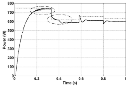
Figure 1. Photovoltaic output power of the conventional P&O approach
