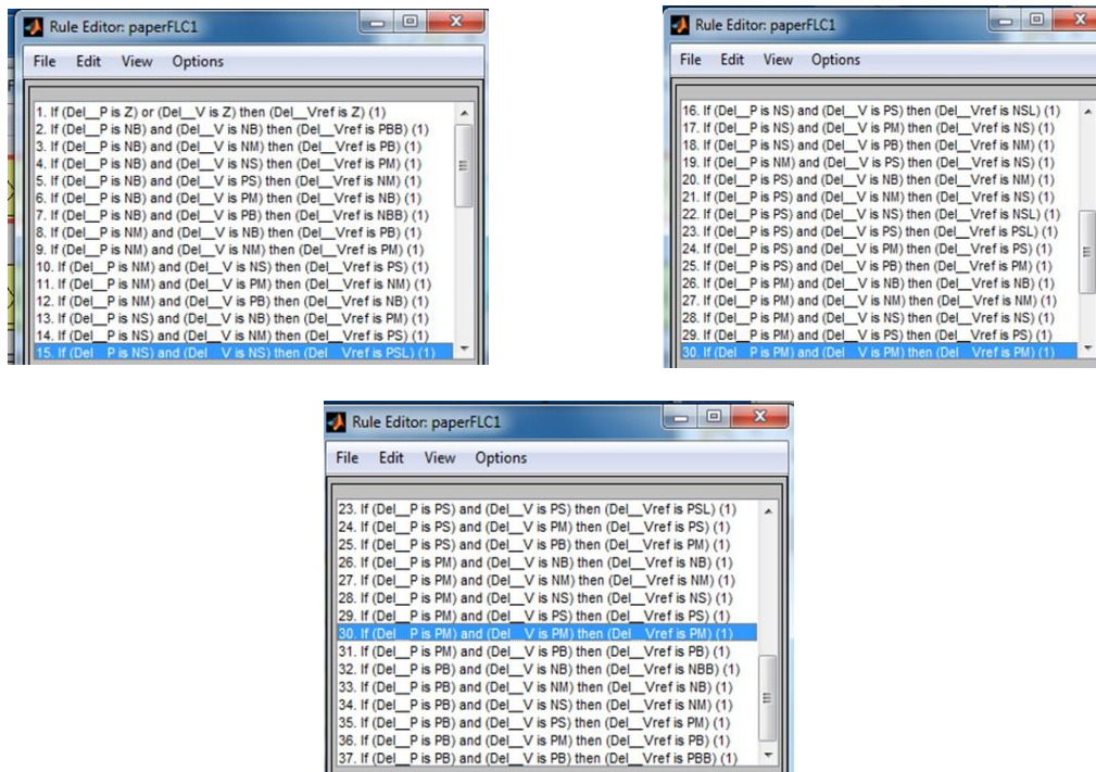
Figure 5. Fuzzification of the improved perturb and observe rules
