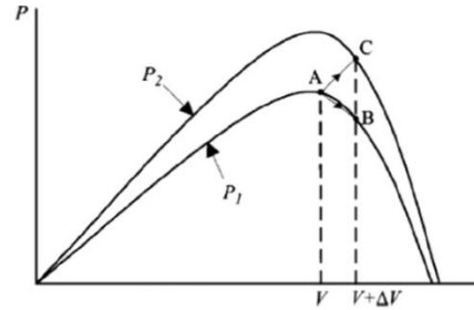
Figure 2. Variance of conventional P&O from MPE as shown in
