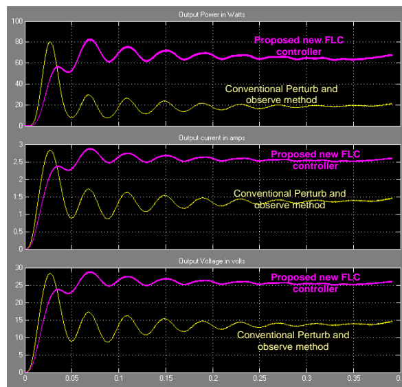
Figure 9. Converter output waveform of power, current and voltage under constant irradiation conditions
