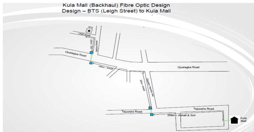
Figure 2. Fiber backhaul connection
