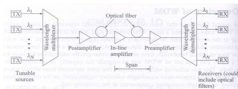
Figure 1. Diagrammatical Representation of Optical Fiber Communication System [1]
