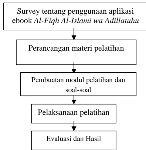
Gambar 8. Persiapan Penelitian
