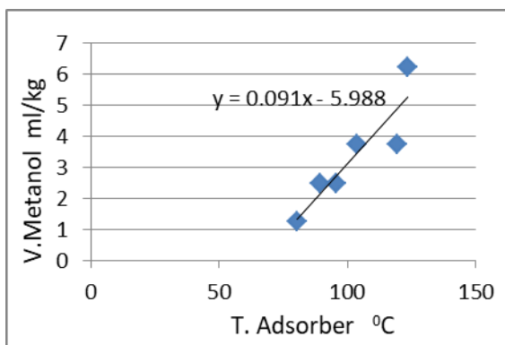
Gambar 4 : Temperatur Adsorber Vs Metanol
