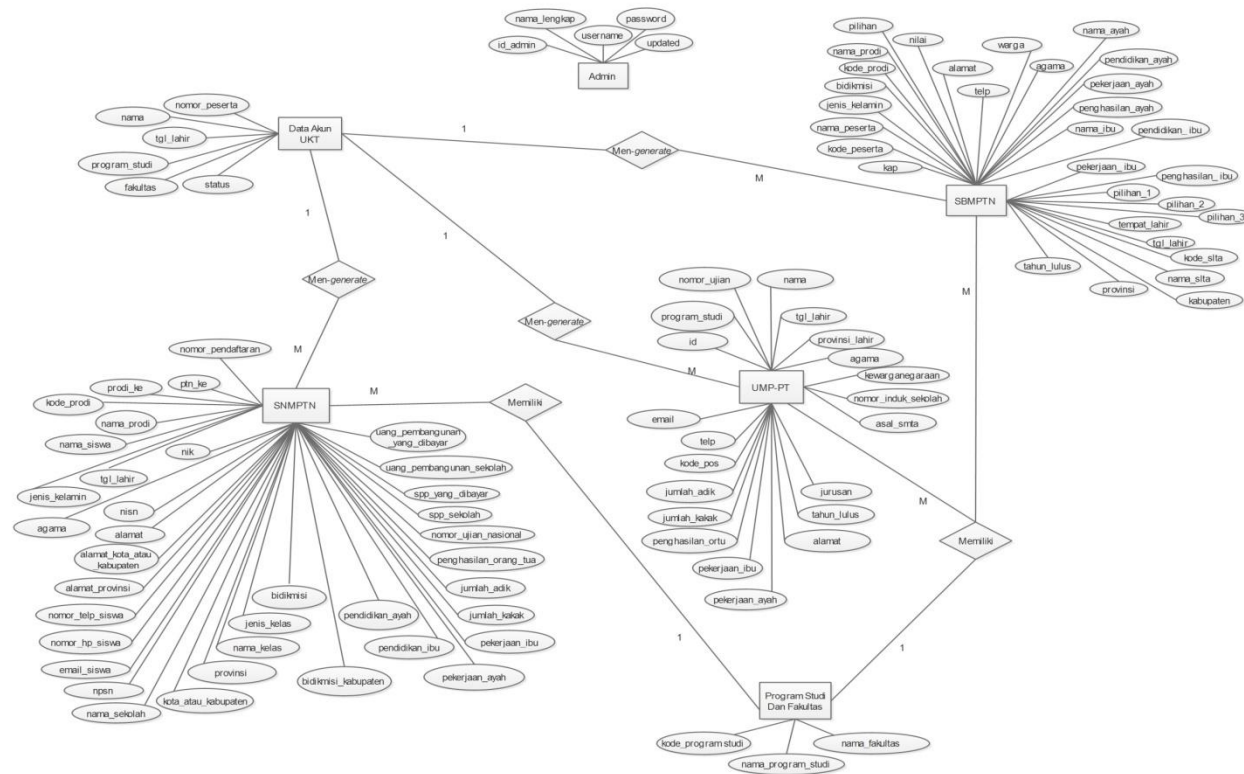
Gambar 4.3 ERD
