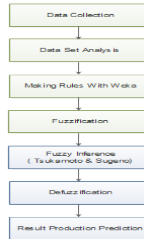
Figure 3.1 Development System
