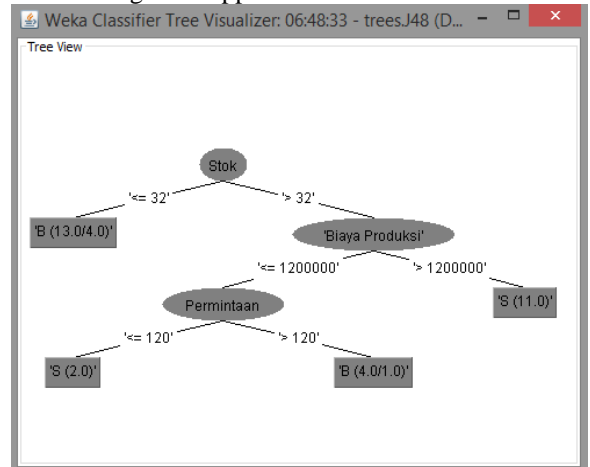
Figure 4.2 Decision Tree
