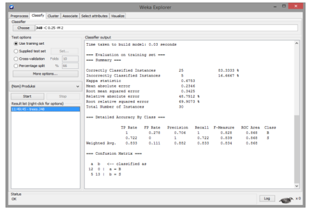
Figure 4.1 Classifier output
