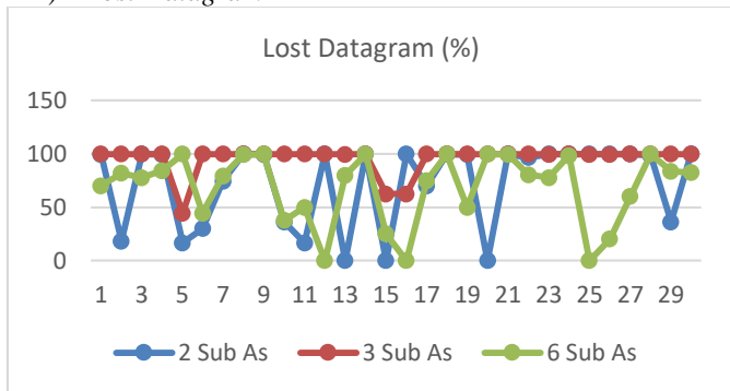
Figure 12. Graphic of Lost Datagram Comparison of Every Sub AS
