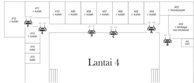
Figure 6. 4 th floor Access Point Installation mapping
