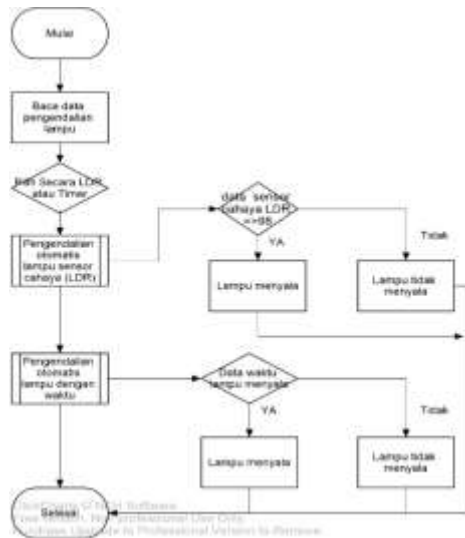
Gambar 6 Flowchart sistem otomatis
