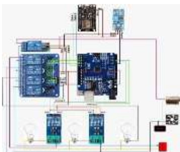
Gambar 7 Wiring diagram Sistem
