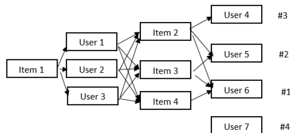
Fig. 1. Item-Based Collaborative Filtering
