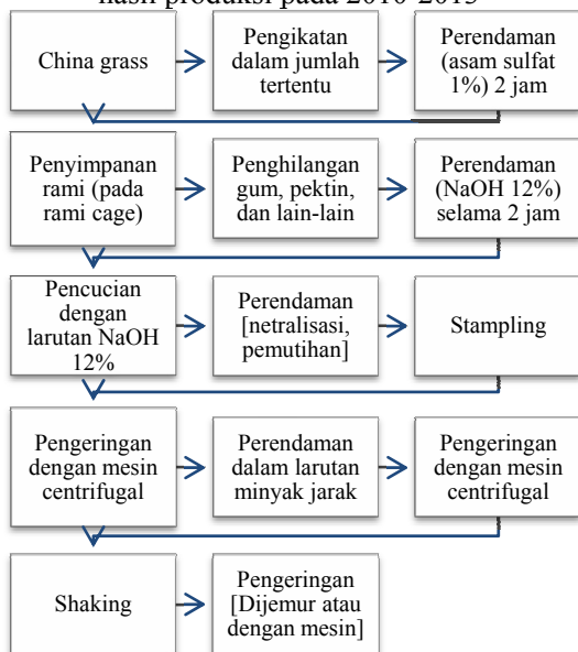
Gambar 5. Tahapan proses degumming
