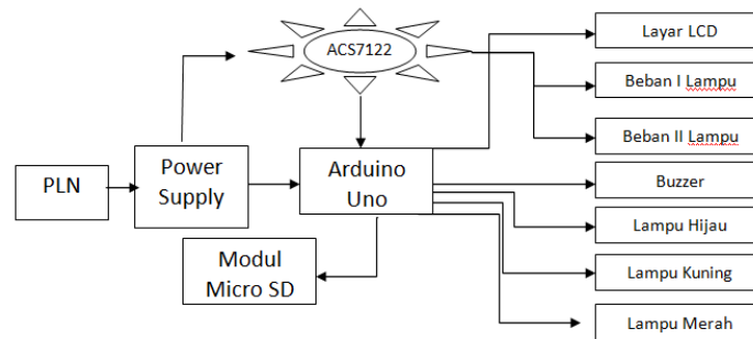
Gambar 1. Diagram Blok Sistem Monitoring Daya Listrik
