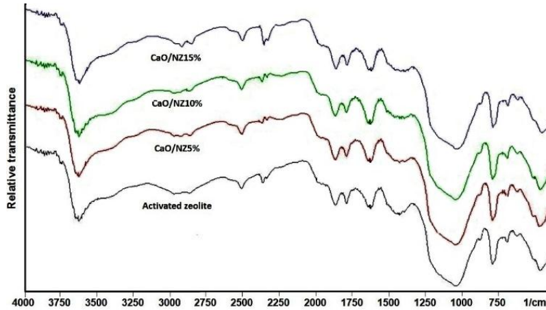
Gambar 3. Spektra FTIR katalis CaO/zeolit alam
