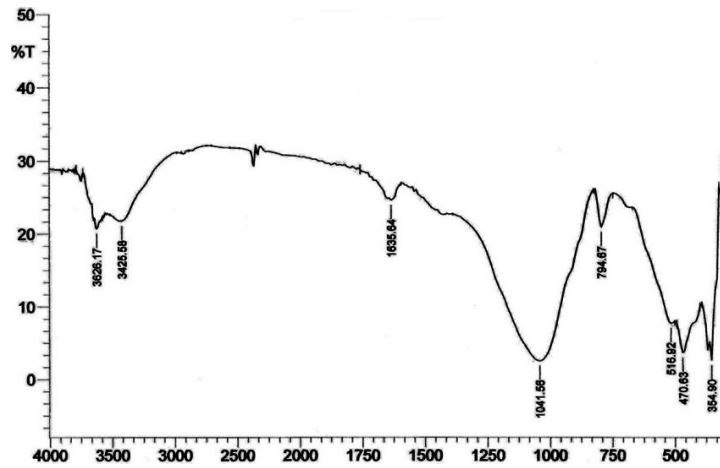
Gambar 1. Spektra FTIR zeolit alam
