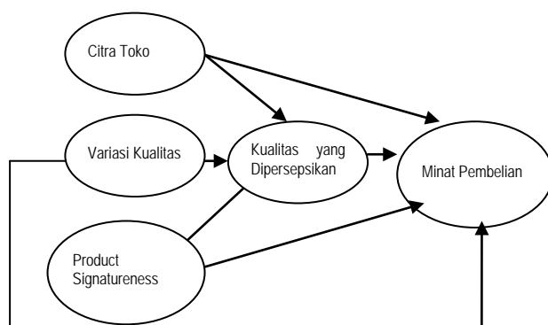
Gambar 3.1 Model Konseptual
