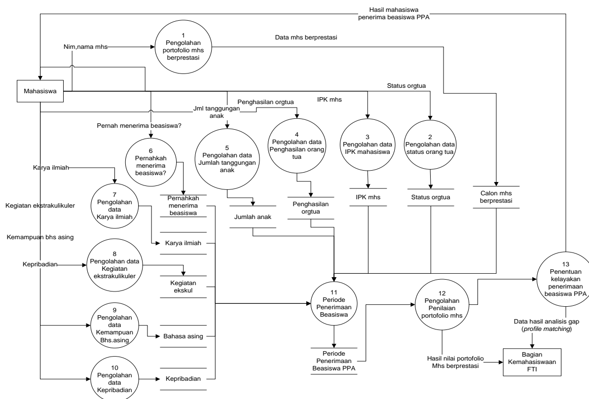
Gambar 2. DFD Level 0
