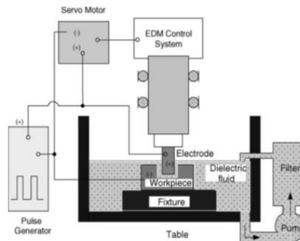
Gambar.1 Skema proses EDM sinking (Lin et al. 2002)
