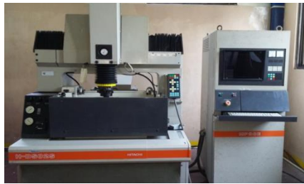
Gambar 6. Mesin EDM sinking H-DS02-S
