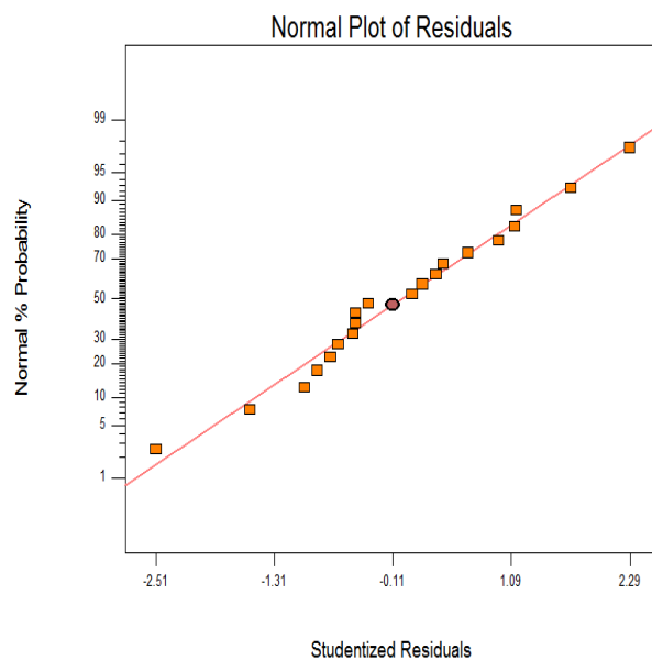
Gambar 8. Normal plot of residuals kekasaran permukaan
