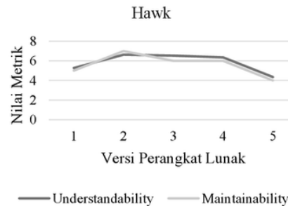
Grafik 3 Nilai Understandability dan Maintainability Hawk
