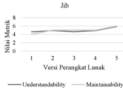
Grafik 2 Nilai Understandability dan Maintainability Jib
